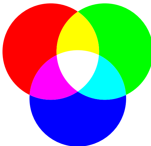
Figure 234: The “color wheel” for screens
